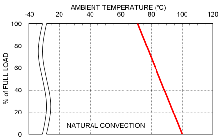
UFED40-48S05W Derating Curve
